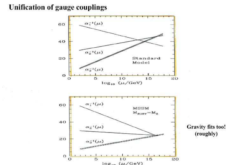
Figure 10: We can test the hypothesis that the disparate coupling strengths of the different gauge interactions derive a common value at short distances, by doing calculations to take into account the effect of virtual particle clouds [16]. These are the same sort of calculations that go into Figure 3, but extrapolated to much higher energies, or equivalently shorter distances. Top panel: using known virtual particles. Bottom panel: including also the virtual particles required by low-energy supersymmetry [17].
